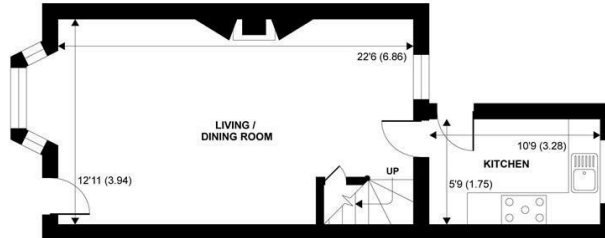
GROUND FLOOR
